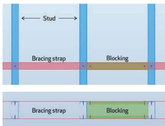
Figure 3.2 Typical 'blocking and bracing'
