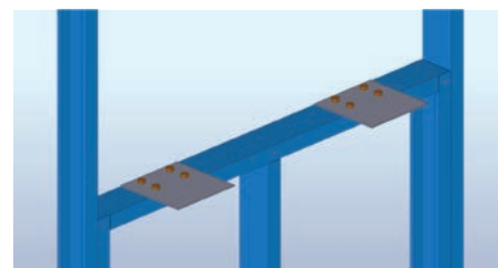
Figure 9.3 Projecting window support brackets fixed to cill
